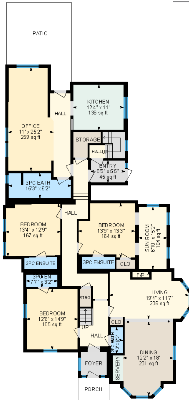
Main Floor Exterior Area 2505.41 sq ft
